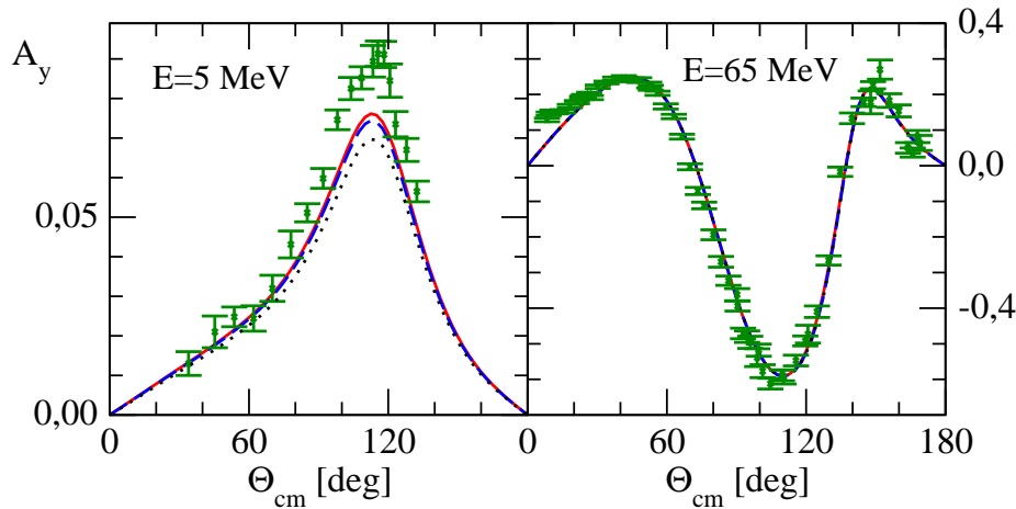
Fig. 2 (Color online) The nucleon analyzing power A_y for nd elastic scattering at 5 MeV and 65 MeV lab. energy of the incoming neutron. The solid (red) line is the nonrelativistic CD Bonn potential prediction. The dashed (blue) and dotted (black) lines are CD Bonn based relativistic predictions without and with Wigner spin rotations, respectively. The 5 MeV nd data (x-es) are from [20] and 65 MeV pd data (x-es) are from [21].
