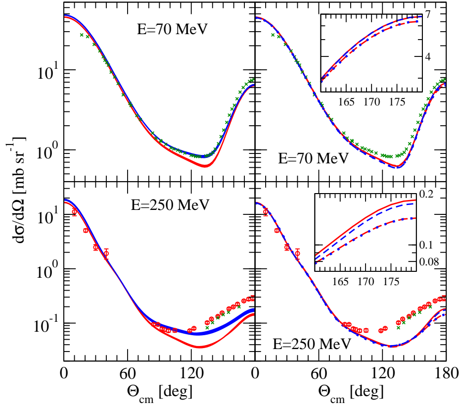
Fig. 1 (Color online) The Nd elastic scattering cross sections at 70 MeV and 250 MeV lab. energy of the incoming nucleon. In the left column predictions based on AV18 [13], CD Bonn [14], NijmI and Nijm II [15] NN potentials alone and on their combinations with the TM99 3NF [16] are shown by the light shaded (red) and dark shaded (blue) band, respectively. In the right column the relativistic predictions based on the boosted CD Bonn ((red) solid line) and AV18 ((blue) dashed line) potentials are compared with the nonrelativistic CD Bonn ((red) dashed line) and AV18 ((blue) dotted line) predictions. The 70 MeV pd data (x-es) are from [17]. The 250 nd (x-es) and pd (open circles) data are from [18] and [19], respectively.
