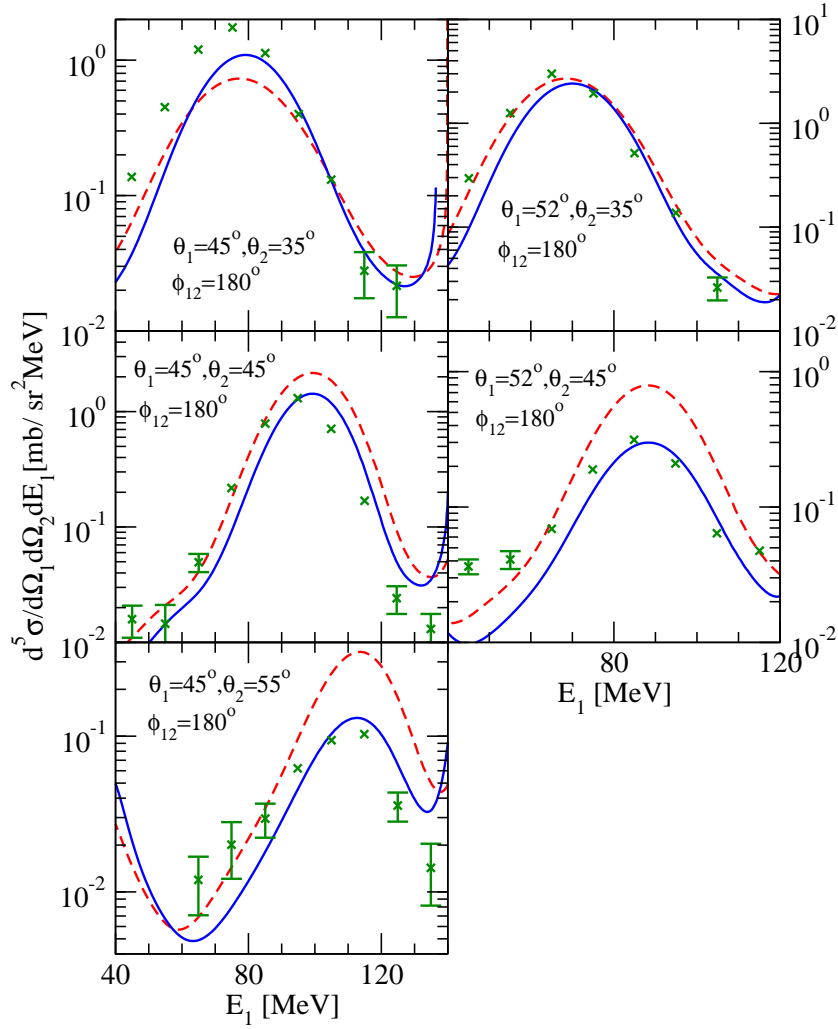
Fig. 3 (Color online) The five-fold cross section d^5\sigma/d\Omega_1 d\Omega_2 dE_1^{lab} for the breakup reaction d(n,np)n at E_{lab} = 200 MeV and fixed angles of outgoing nucleons 1 and 2 as indicated in the figures. The dashed (red) line is the nonrelativistic CD Bonn potential prediction and the solid (blue) line is the corresponding relativistic result. The d(p,pn)p data (x-es) are from [22].
