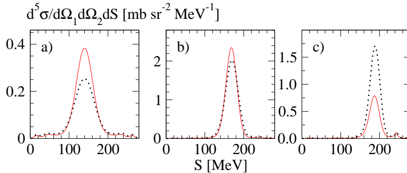
Figure 2. Cross sections for exclusive d(n,nn)p breakup at E_{lab}^n = 200 MeV at a fixed angle \theta_2 = 37.5^\circ and varying \theta_1 : a) \theta_1 = 37.5^\circ , b) \theta_1 = 47.5^\circ , c) \theta_1 = 57.5^\circ . The non relativistic (relativistic) cross sections based on CD Bonn are shown by dashed (solid) lines, respectively.
