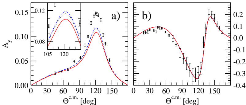
Figure 1. The nucleon analyzing power A_y in elastic Nd scattering at E_{lab}^N = 8.5 MeV (a) and 35 MeV (b). The dashed line is the non relativistic result obtained with the CD Bonn potential. The relativistic predictions are given by the dotted (without) and solid lines (with) Wigner rotations, respectively. The nd data in a) are from [7] and pd data in b) from [8].
