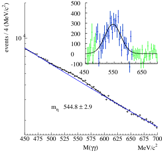
FIG. 1: M(\gamma\gamma) distribution for photon pairs in the \eta mass region. Results for the fit shown are in Table I. The inset shows the background subtracted \eta signal. The dark points indicate the \eta signal region.
