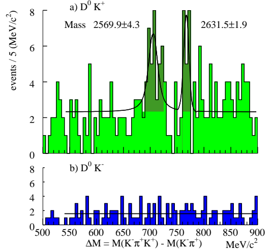
FIG. 3: (a) D_s(2632) \rightarrow D^0K^+ mass difference distribution. Charged conjugates are included. The shaded regions are the event excesses used in the estimation of signal significances. Results for the fit shown are in Table I. (b) Wrong sign background D^0K^- events, as described in the text.
