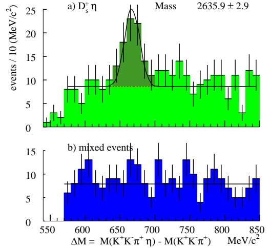
FIG. 2: (a) M(KK\pi^\pm \eta) - M(KK\pi^\pm) mass difference distribution. Charged conjugates are included. The shaded region is the event excess used in the estimation of signal significance. Results for the fit shown are in Table I. (b) Mass difference distribution for mixed events as described in the text.
