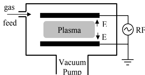
FIGURE 2. Schematic diagram of the rf driven parallel plate GEC reference cell.
