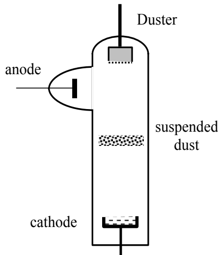
FIGURE 3. DC glow discharge device (positive column) for dusty plasma studies.
